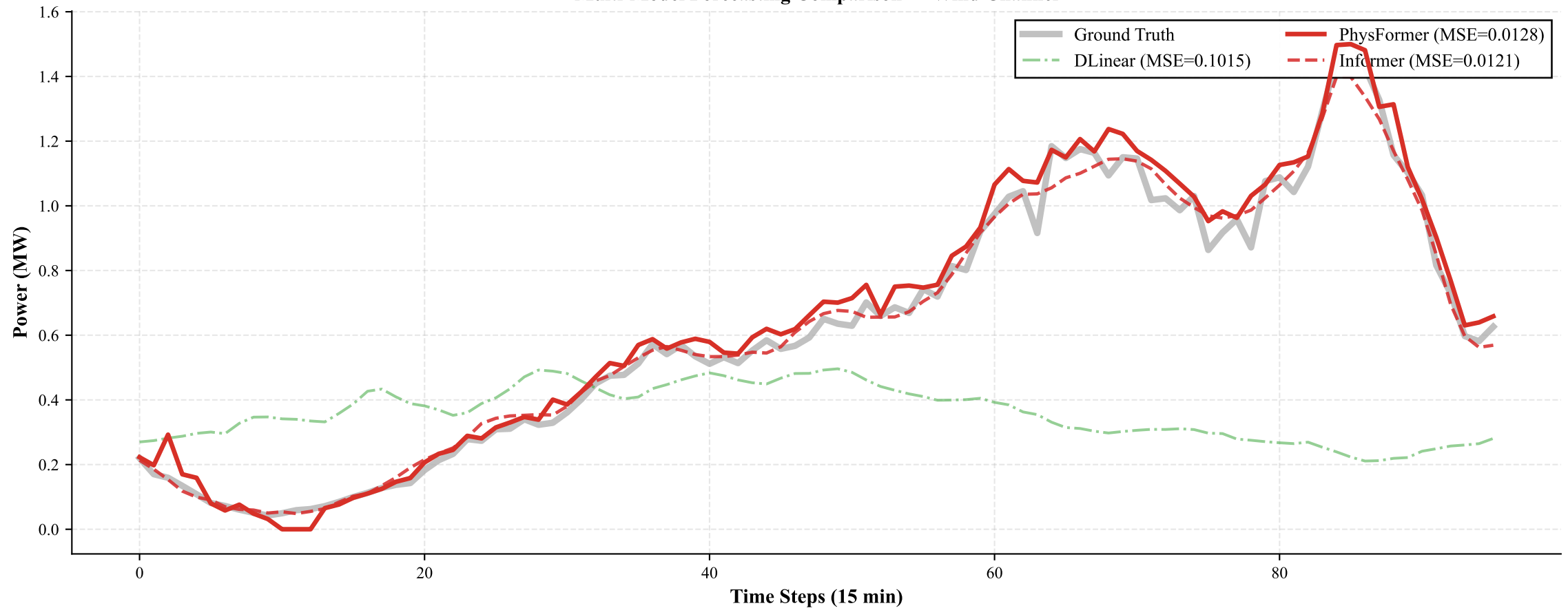
Multi-Model Forecasting Comparison — Wind Channel
